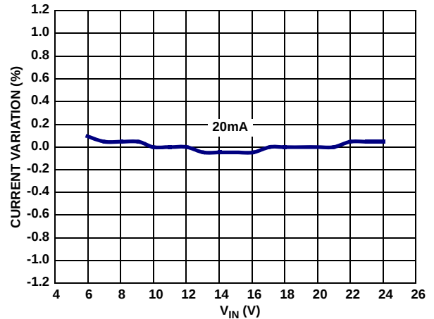
FIGURE 5. CURRENT REGULATION
