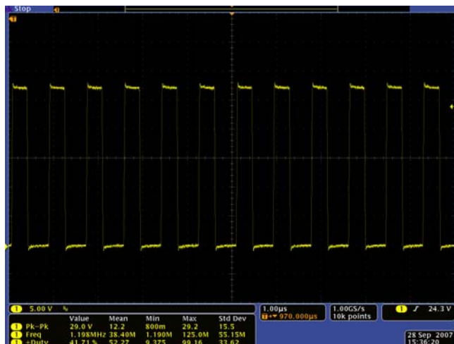
FIGURE 14. LX ZOOM IN AT 50% DIMMING (54 LEDs, 20mA, V_{IN} = 12V )
