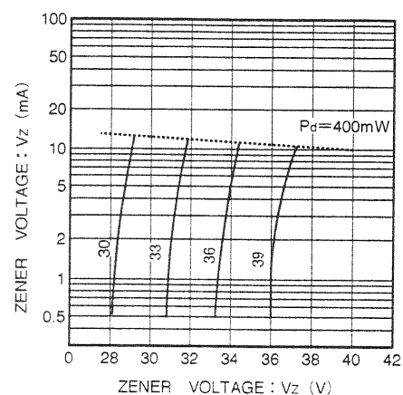
Fig. 3 RLZ30 ~ RLZ39 Zener characteristic
