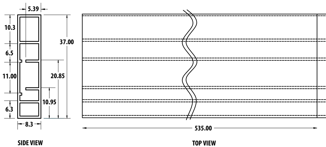
Figure 15. Tube dimensions
