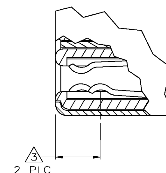
DETAIL D SCALE 10:1
