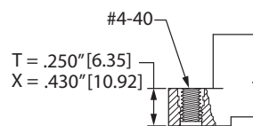
FLUSH MOUNTING WITH THREADED INSERT (T, X)
