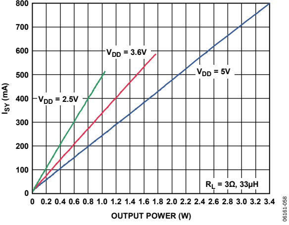
Figure 37. Supply Current vs. Output Power into 3 \Omega
