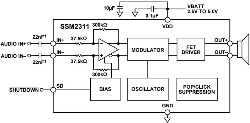
Figure 43. Differential Input Configuration
