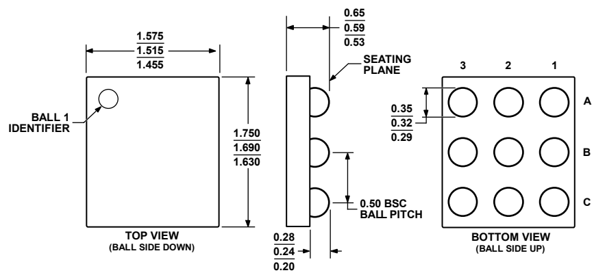
Figure 48. 9-Ball Wafer Level Chip Scale Package [WLCSP] (CB-9-1) Dimensions shown in millimeters
