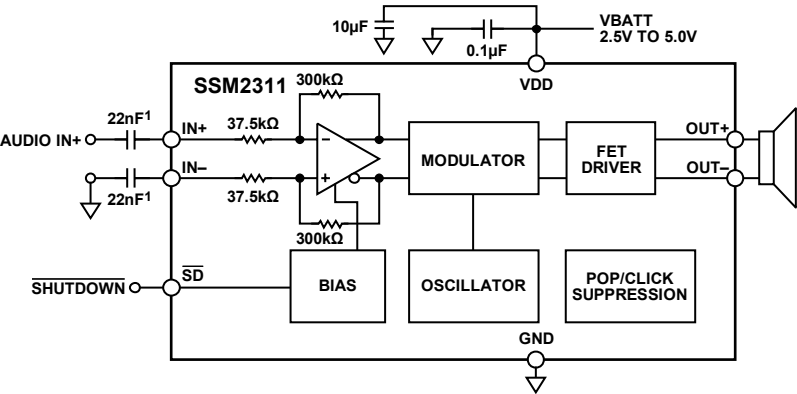
Figure 44. Single-Ended Input Configuration
