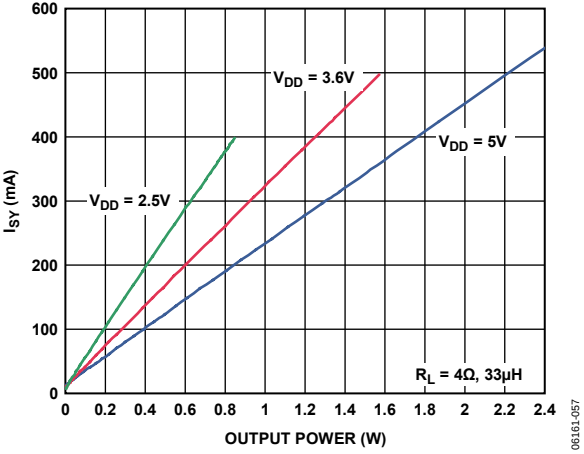
Figure 36. Supply Current vs. Output Power into 4 \Omega
