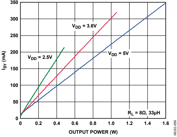
Figure 35. Supply Current vs. Output Power into 8 \Omega
