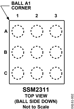
Figure 2. SSM2311 WLCSP Pin Configuration
