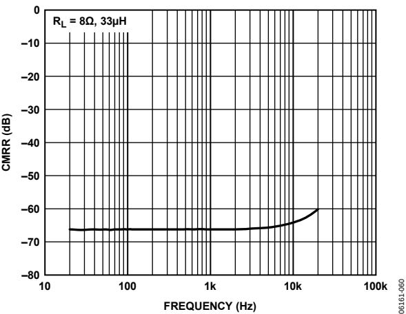
Figure 39. Common-Mode Rejection Ratio vs. Frequency
