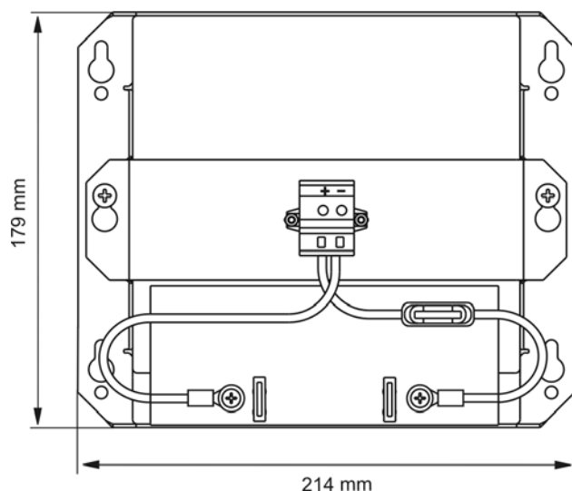
Fig. 1 Front view
