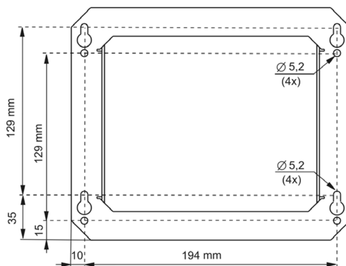
Fig. 2 Hole pattern
