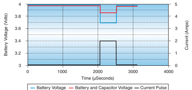
Figure 5. GSM Pulse
