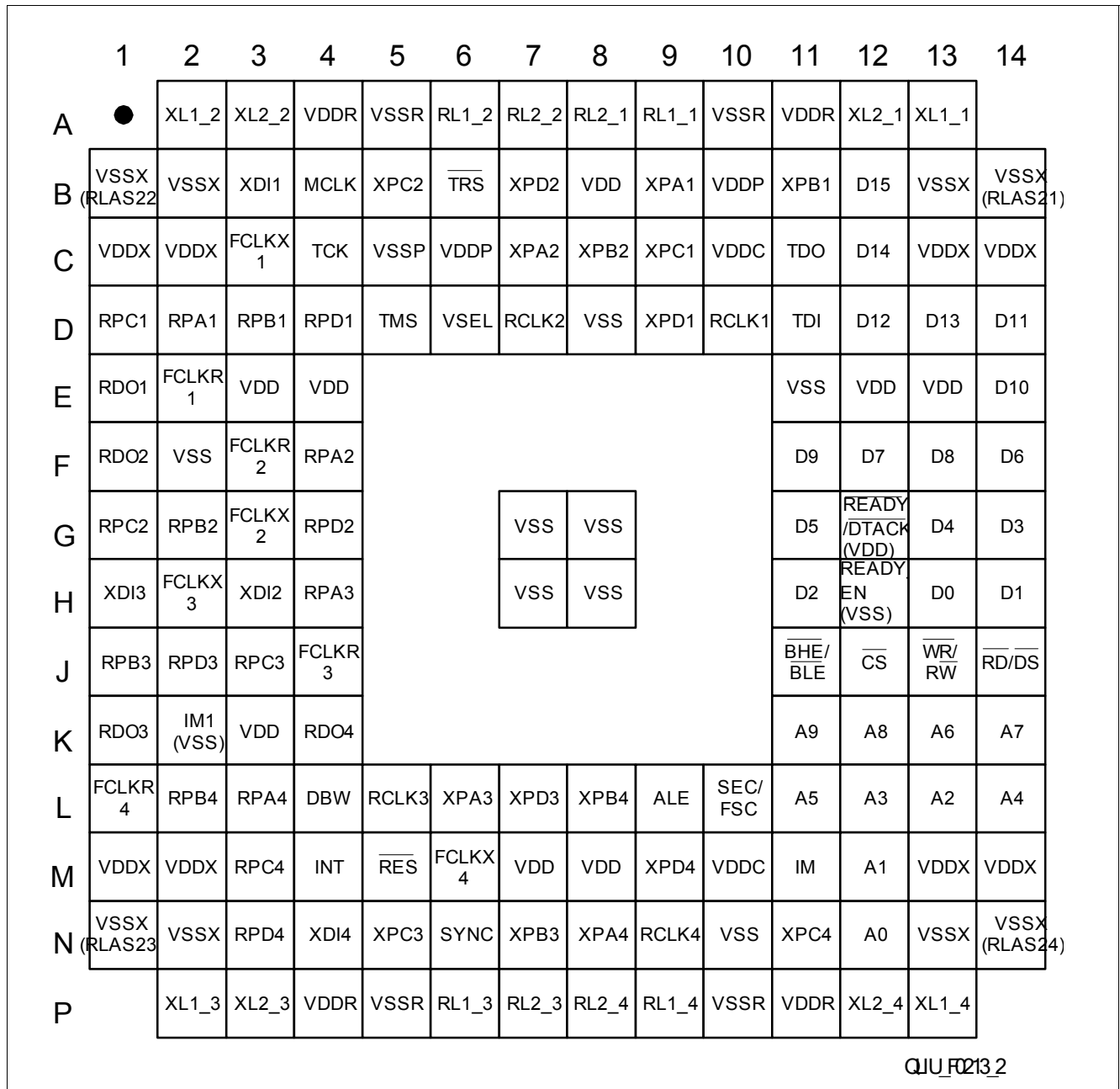
Figure 4 Top View of the Pin Configuration (Ball Layout) P/PG-LBGA-160-1
