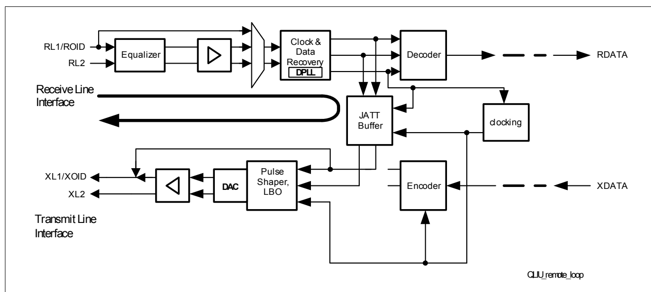
Figure 43 Remote Loop
