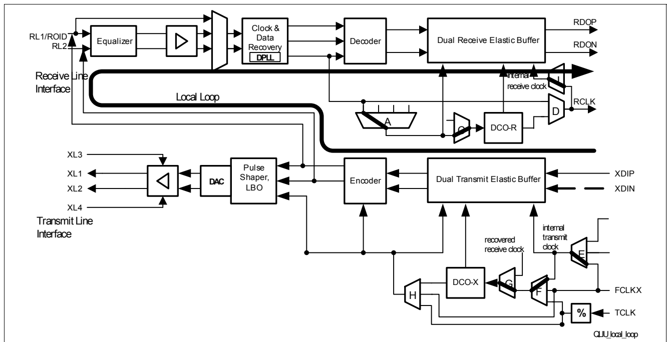
Figure 44 Local Loop
