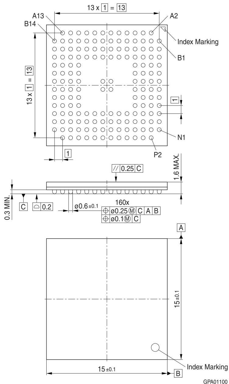
Figure 46 P/PG-LBGA-160-1 (Plastic Green Low Profile Ball Grid Array Package)
