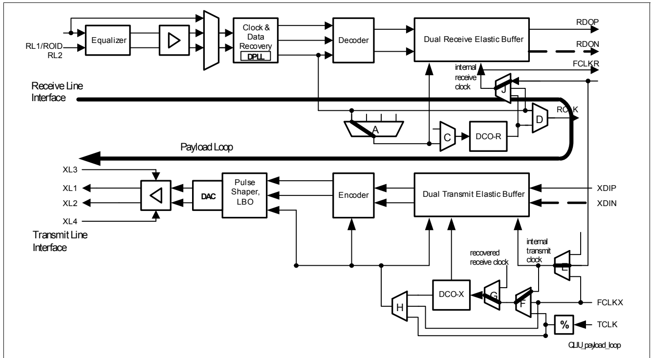
Figure 45 Payload Loop
