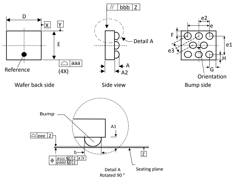
Figure 21. WLCSP8 - Outline
