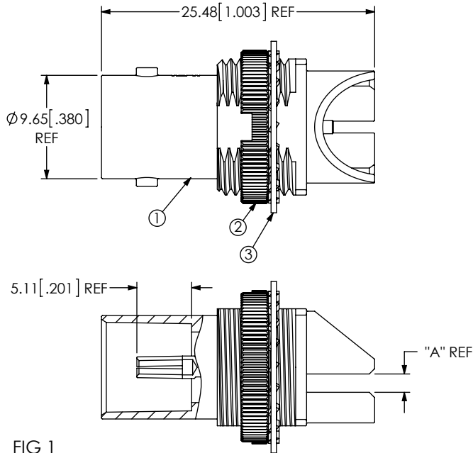
FIG 1 BNC7T-J-P-XX-ST-EM1D SHOWN
