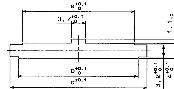
< PANEL CUTOUT >
