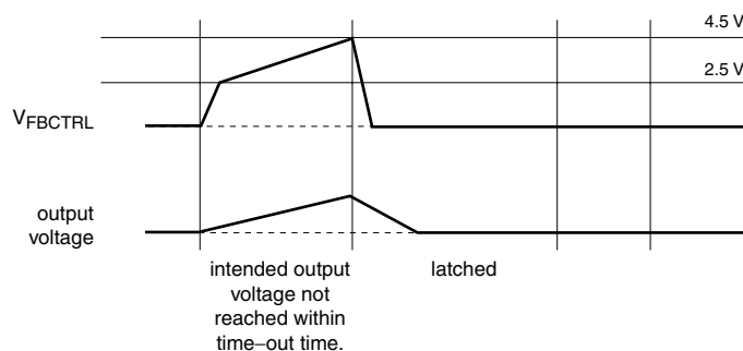
Fig 13. Time-out protection (signals), latched in the TEA1751L
