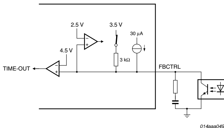
Fig 11. Time-out protection circuit
