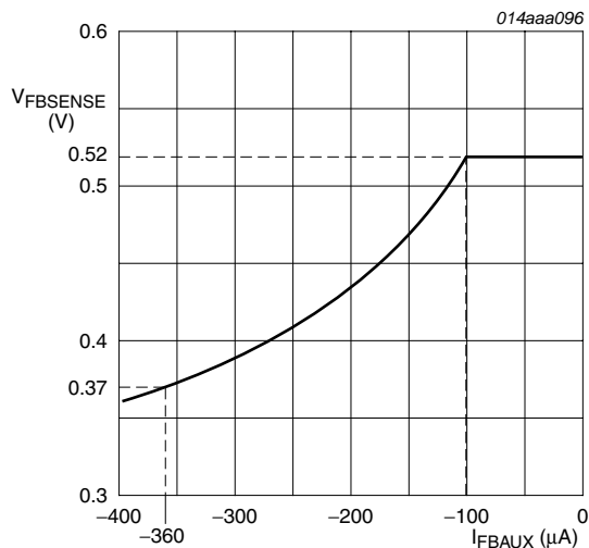
Fig 16. Overpower protection curve
