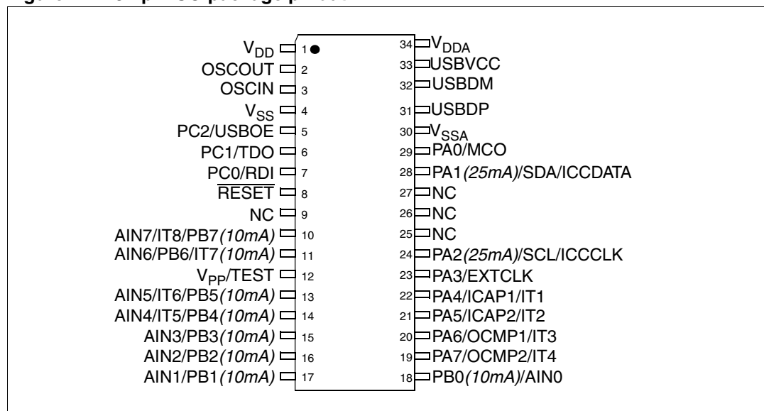
Figure 4. 34-pin SO package pinout
