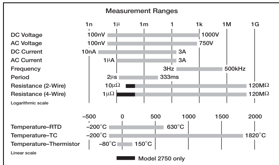
Figure 2. Measurement Ranges
