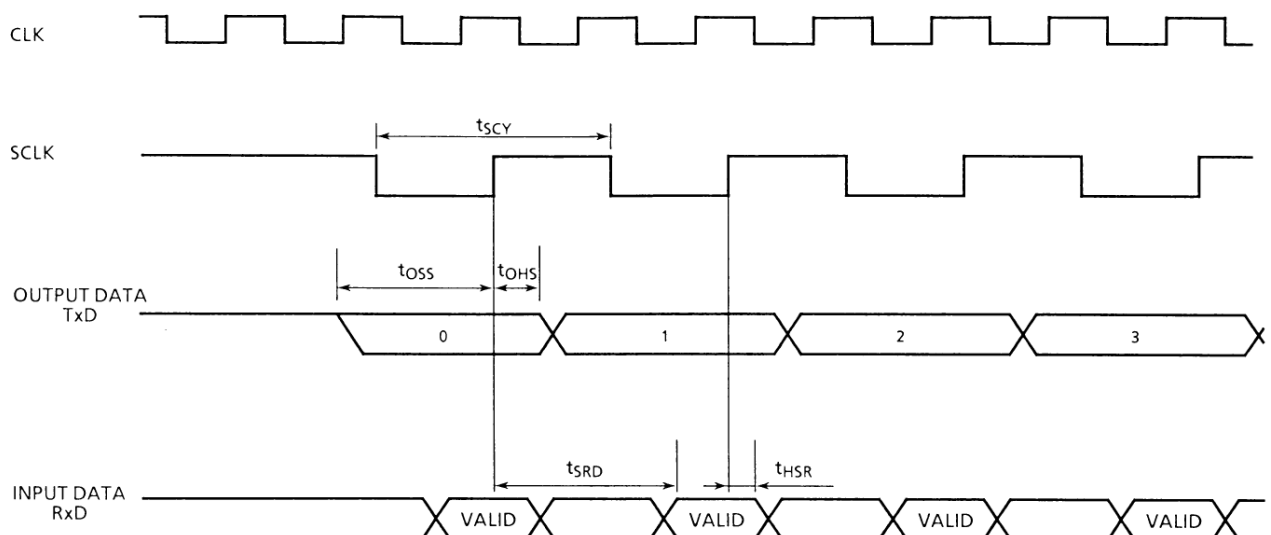
TMP90CM40A I/O Interface Mode Timing Waveforms
