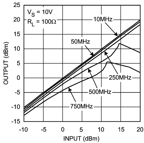
Linearity V_{\text{OUT}} vs. V_{\text{IN}}
