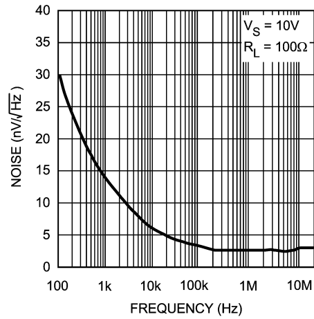
Voltage Noise
