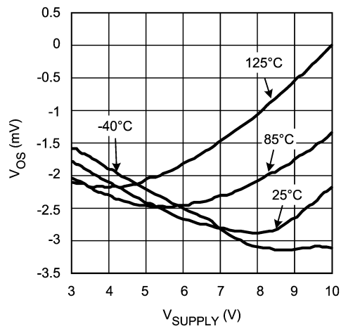
V_{\text{OS}} vs. V_{\text{SUPPLY}} for Unit 1
