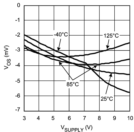
V_{\text{OS}} vs. V_{\text{SUPPLY}} for Unit 2
