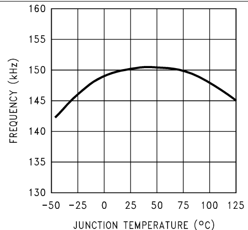
Figure 13. Switching Frequency
