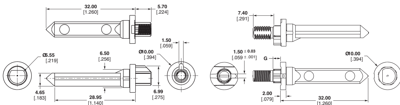
Pin Part Number 1410548-2
