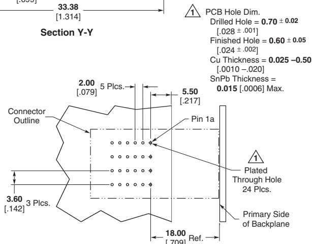
Recommended PCB Hole Layout
