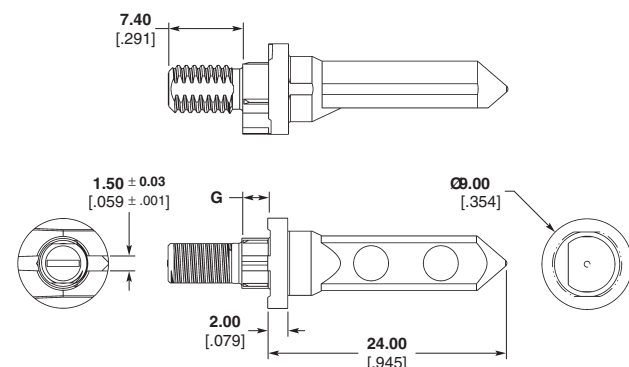
Pin Part Number 1469491-X
