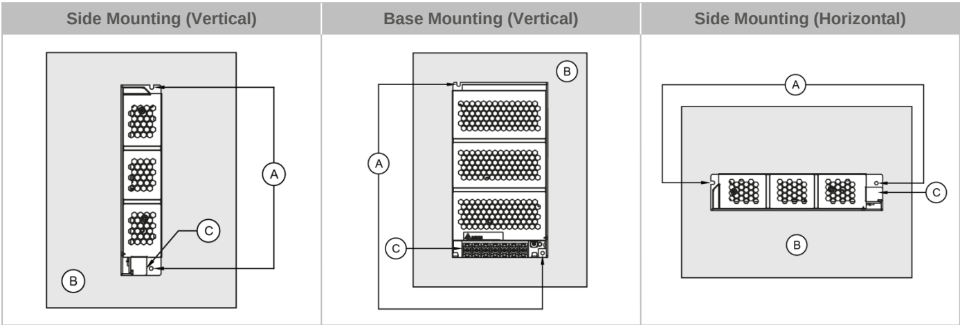
Fig. 2 Mounting Orientation
