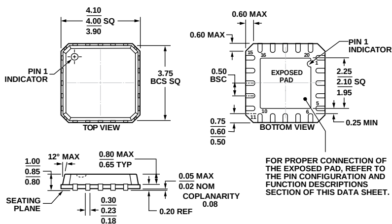
Figure 25. 20-Lead Lead Frame Chip Scale Package [LFCSP_VQ] 4 mm x 4 mm Body, Very Thin Quad (CP-20-1)
