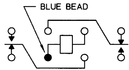
TERMINAL VIEW
