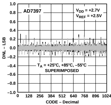
Figure 7. AD7397 DNL vs. Code and Temperature
