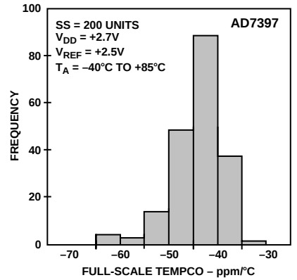
Figure 9. AD7397 Full-Scale Tempco Histogram
