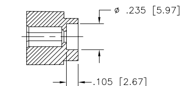
SECTION U-U
