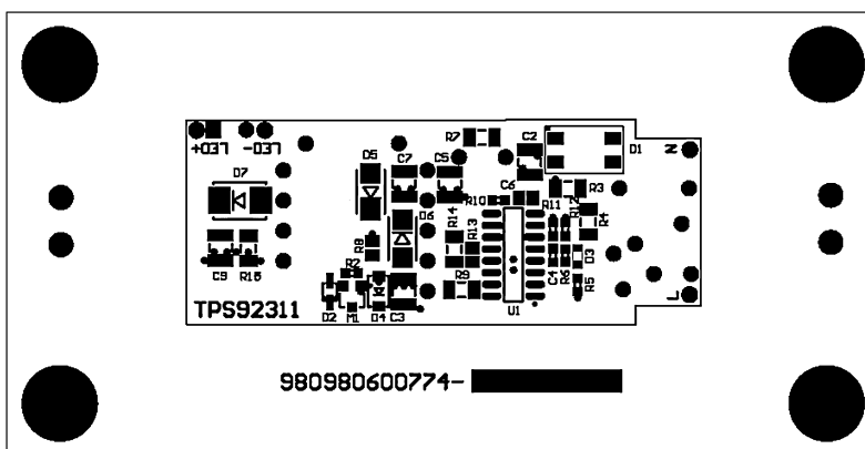
Figure 27. Bottom Layer Assembly Drawing (Bottom View)
