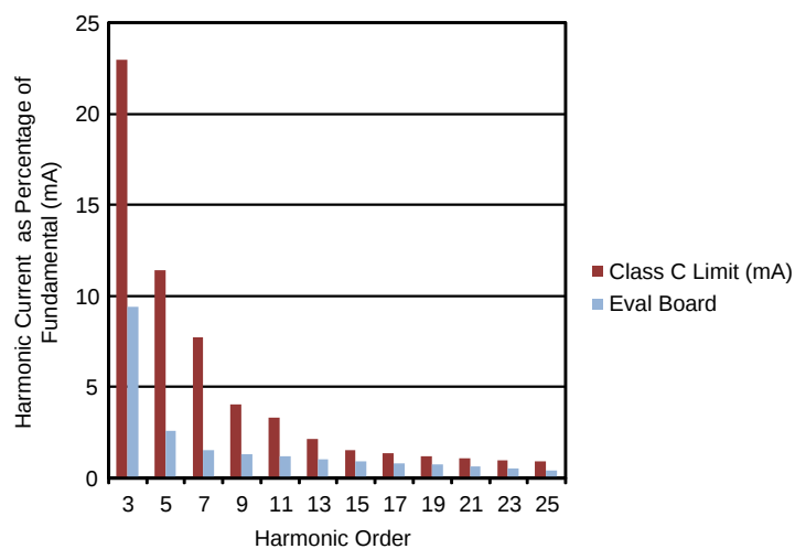
Figure 20. TPS92311 120V EVM Current Harmonic vs IEC61000-3-2 Class C Limits
