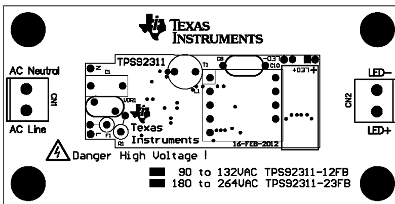
Figure 26. Top Layer Assembly Drawing (Top View)
