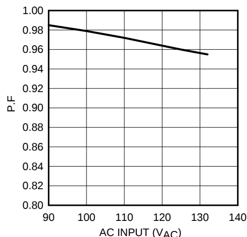
Figure 9. Power Factor
