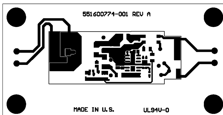
Figure 29. Bottom Layer Copper (Bottom View)
