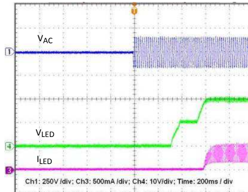
Figure 15. Power Up Output Voltage and Current (120VAC)
