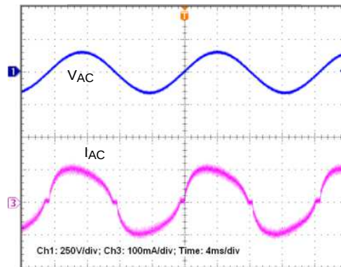
Figure 13. Input Voltage and Input Current (120VAC)
