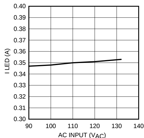
Figure 7. Line Regulation
