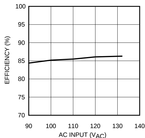
Figure 5. Efficiency vs AC Input
