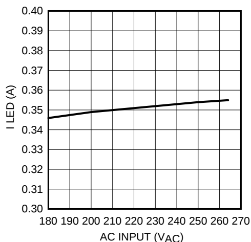
Figure 6. Line Regulation
