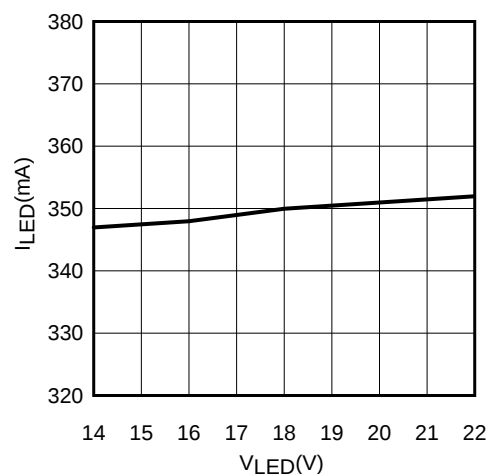
Figure 11. Load Regulation (120VAC)
