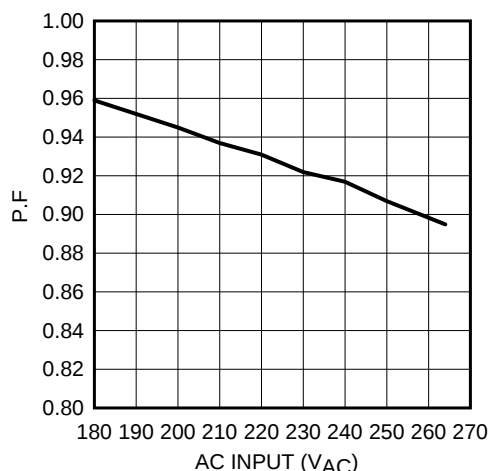
Figure 8. Power Factor
