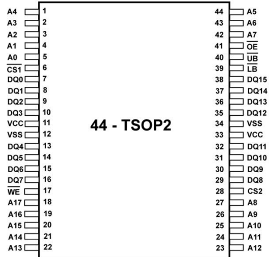
44 - TSOP2 : Top view
