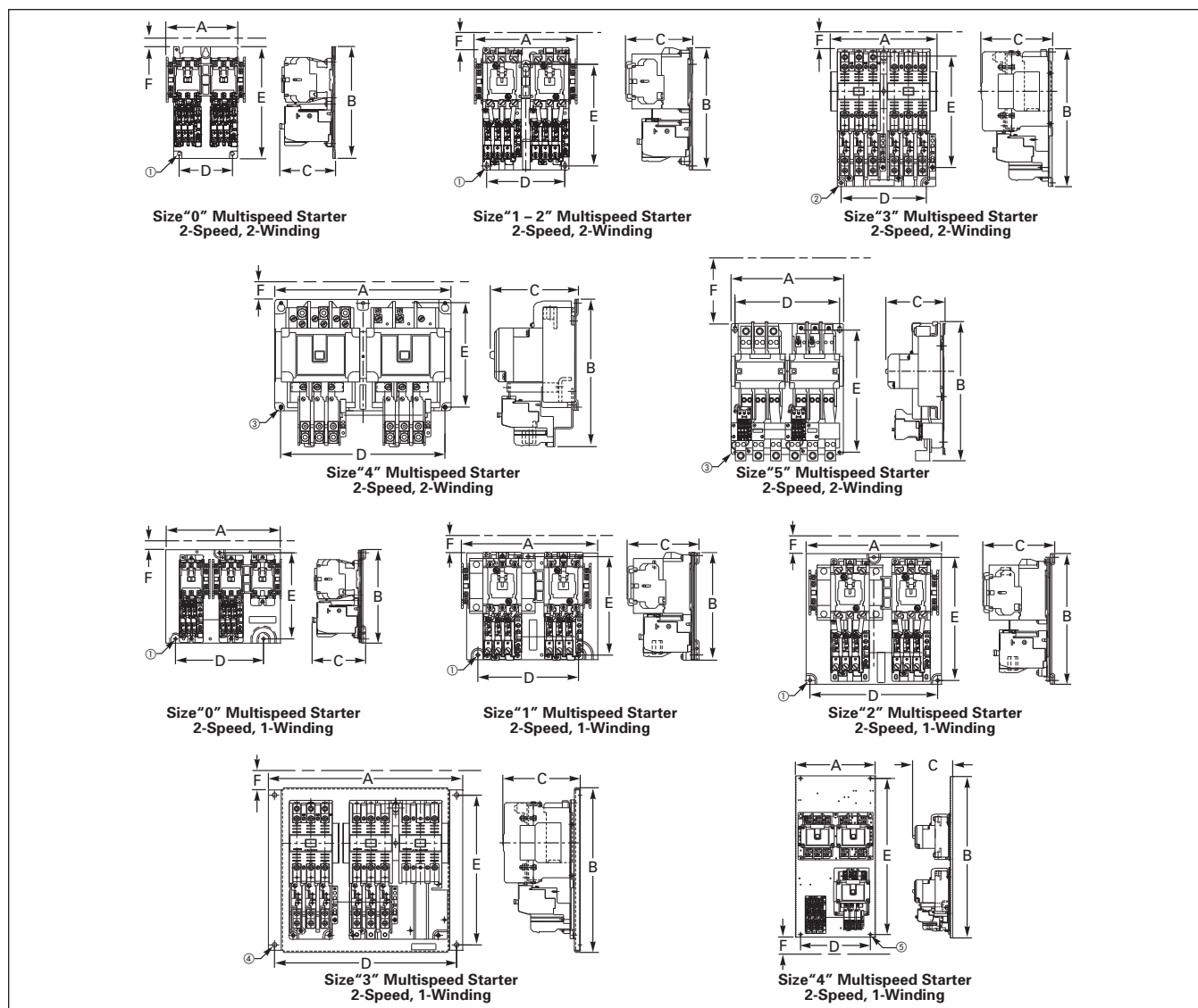
Figure 33-39. Approximate Dimensions
