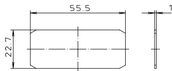
Frontplatte Alu
