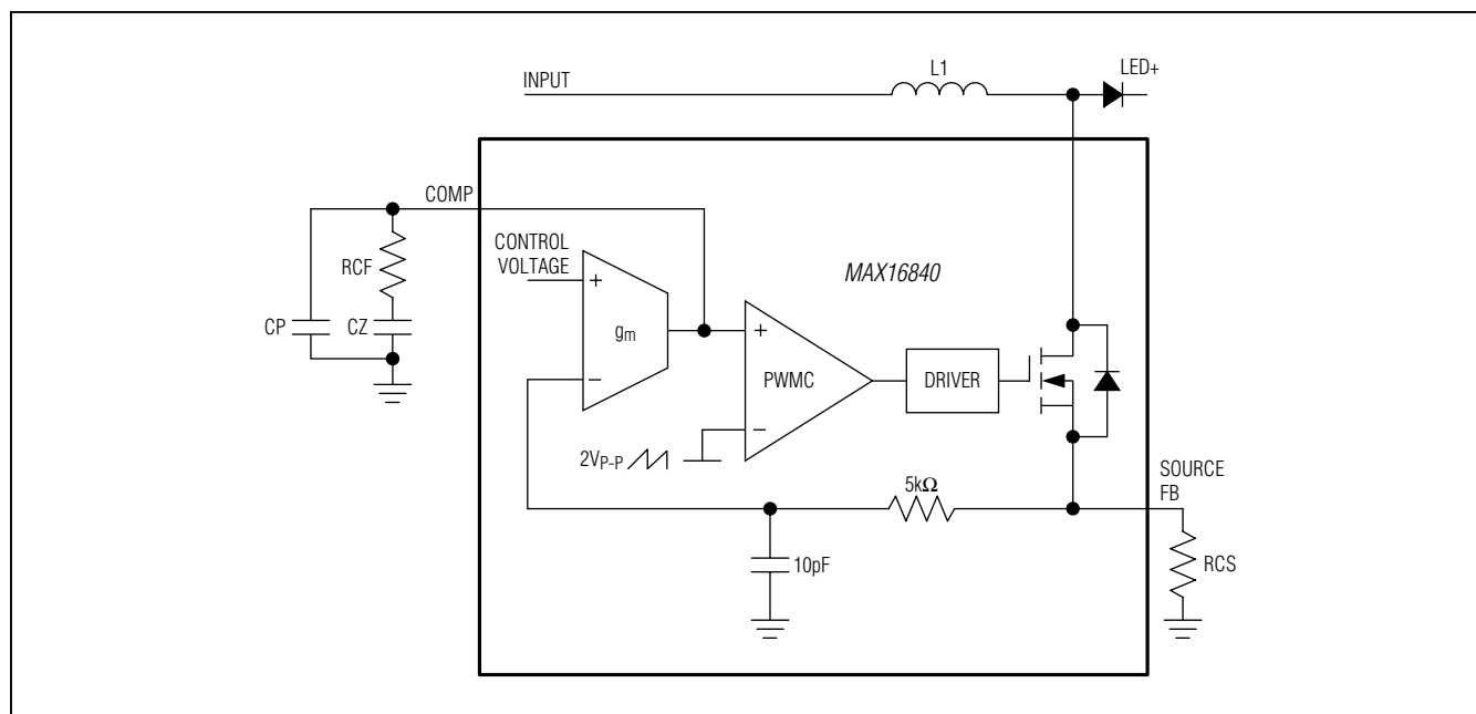
Figure 1. Control Loop
