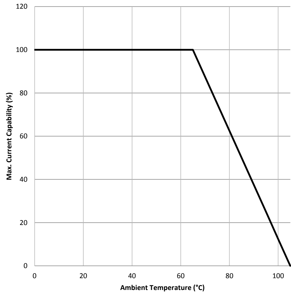
Derating Curve:
