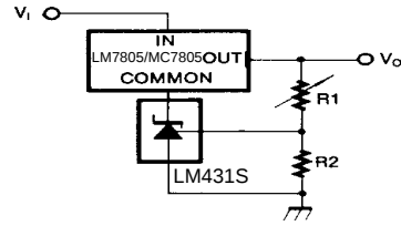
Figure 16. Output for Three-Terminal Fixed Regulator
