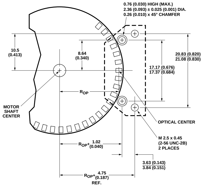
Figure 1. Mounting plane side A.
