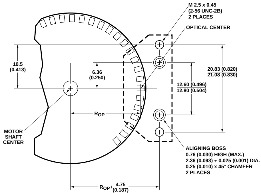
Figure 2. Mounting plane side B.
