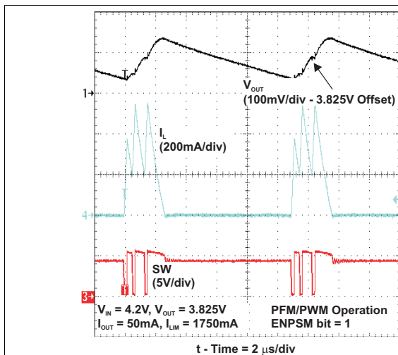
Figure 69. Down-Mode Operation (Voltage Mode)
