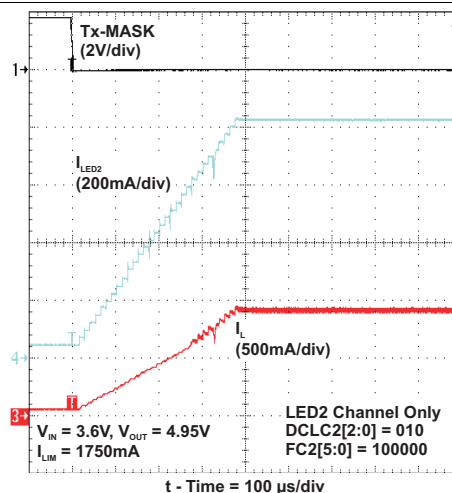
Figure 63. Tx-Masking Operation
