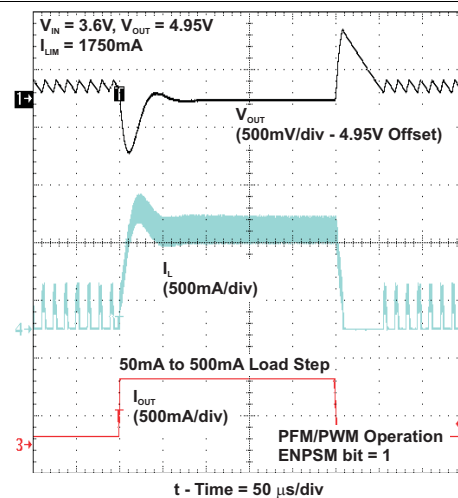
Figure 70. Voltage Mode Load Transient Response
