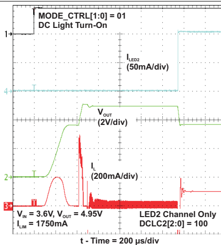
Figure 67. Start-Up Into Video Light Operation
