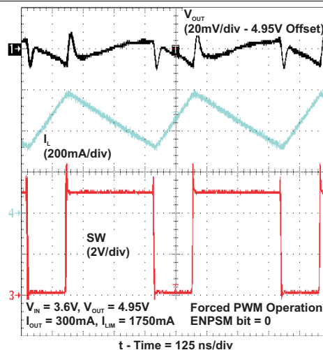
Figure 65. PWM Operation
