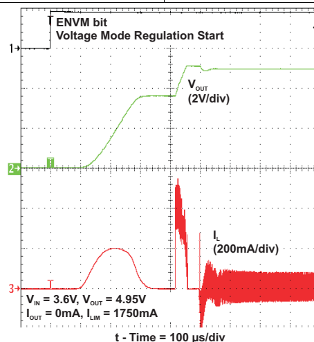
Figure 71. Start-Up Into Voltage Mode Operation
