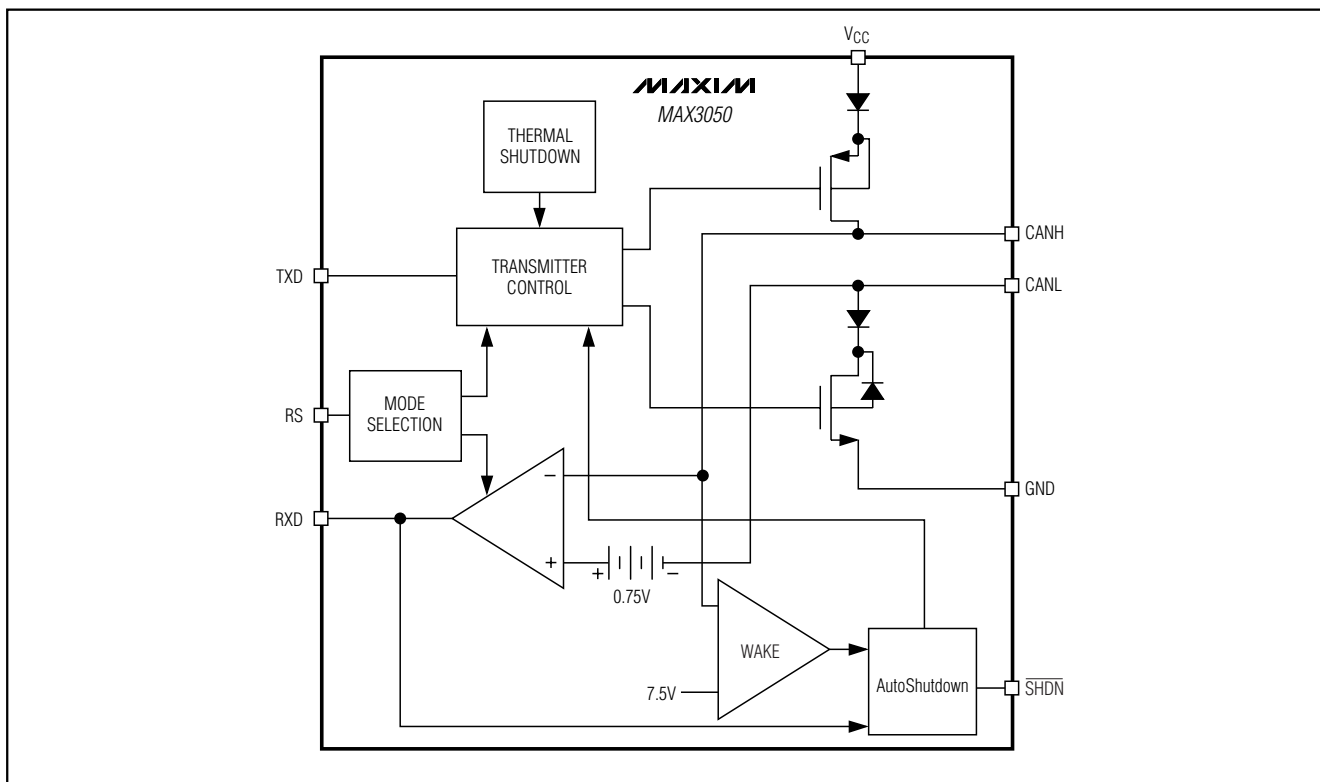
Figure 4. Functional Diagram
