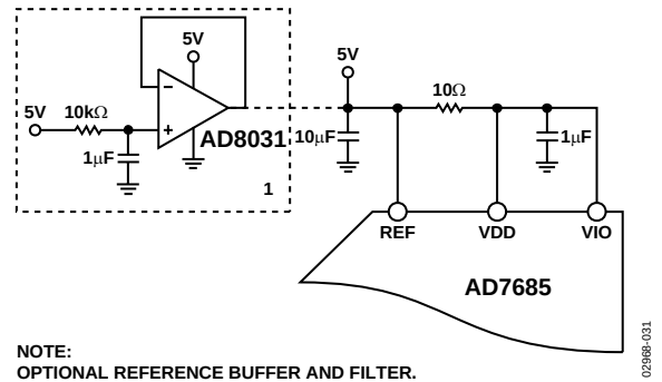
Figure 32. Example of Application Circuit
