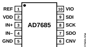
Figure 5. 10-Lead MSOP and QFN 1 (LFCSP) Pin Configuration
