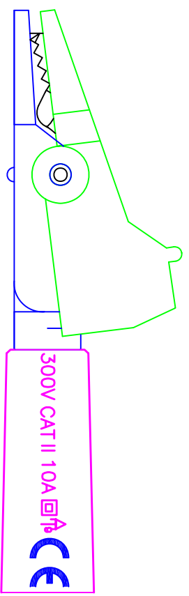
Croc. clip: 116010
