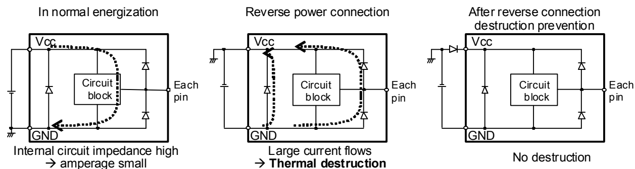
Fig.13 Flow of current when power is connected reversely
