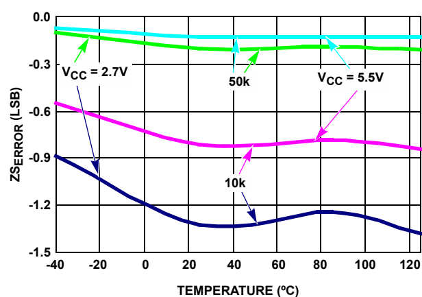
FIGURE 6. ZSERROR vs TEMPERATURE
