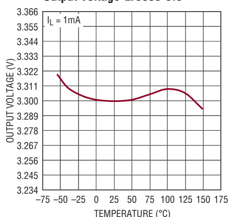
Output Voltage-LT3055-3.3
