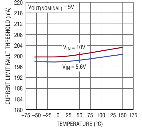
Precision Current Limit, R_{\text{IMAX}} = 1.5\text{k}\Omega
