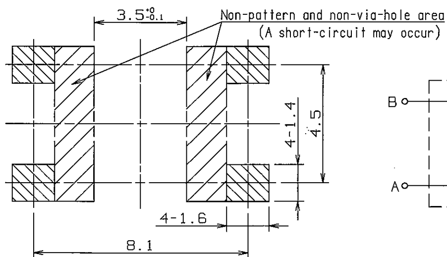
Land Pattern Plan
