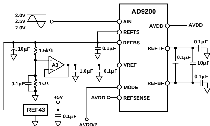
Figure 22. External Reference Mode—1 V p-p Input Span 2.5 V V_{CM}
