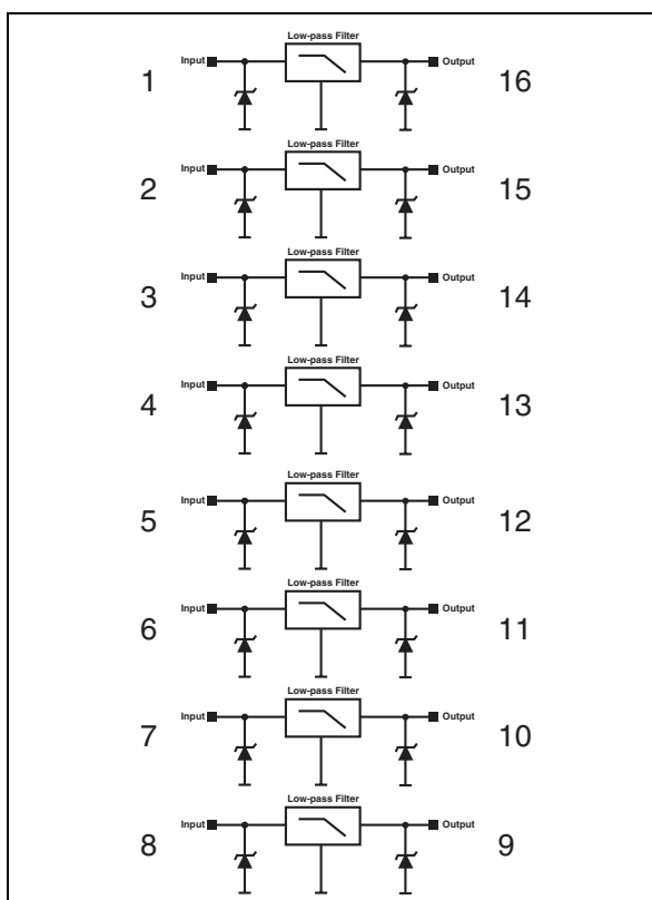
Figure 2: Pin Configuration
