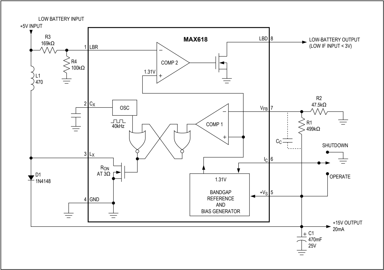
Figure 1. Single-Supply Operation
