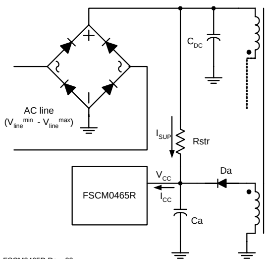
Figure 16. Startup Circuit
