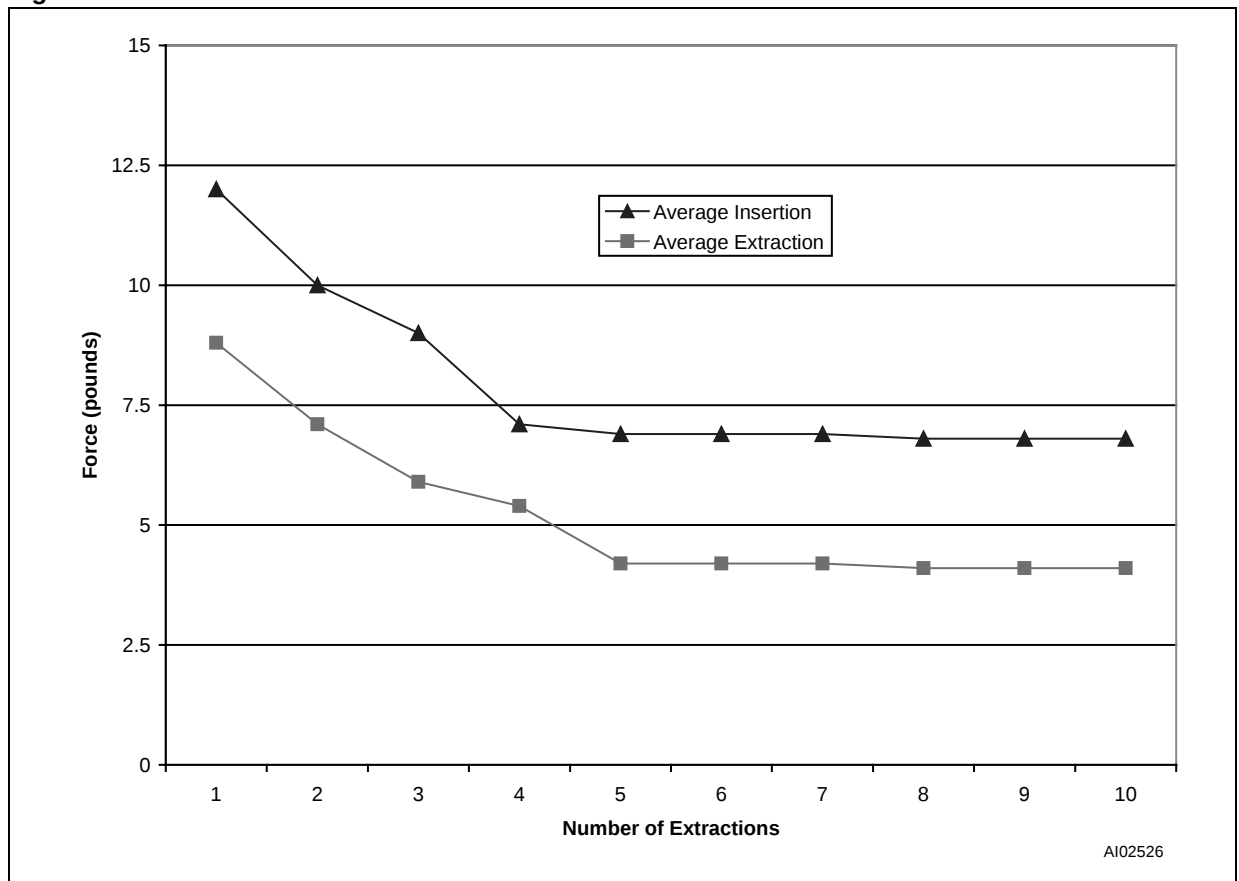
Figure 3. SNAPHAT Insertion/Extraction Forces
