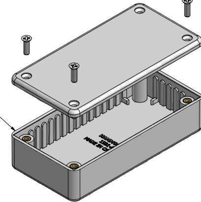
EXPLODED VIEW OF ENCLOSURE
