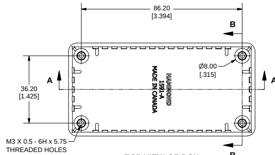
TOP VIEW OF BOX
