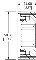
SECTION B-B
