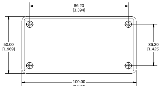
BOTTOM VIEW OF LID
