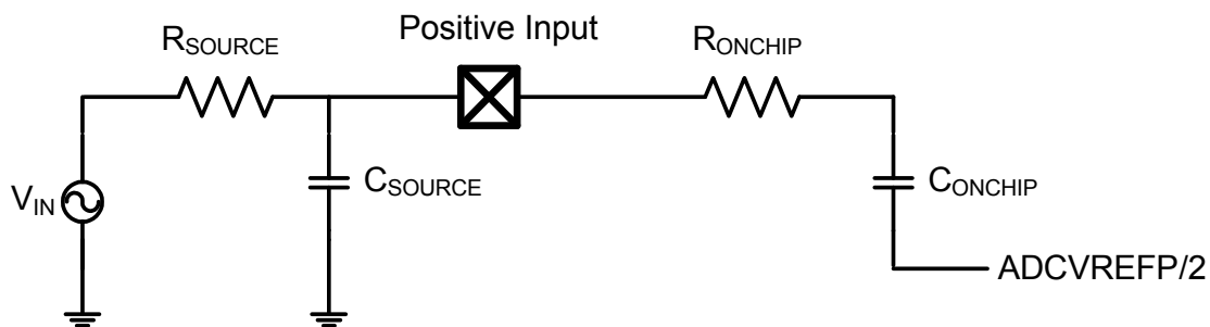
Figure 7-7. ADC Input
