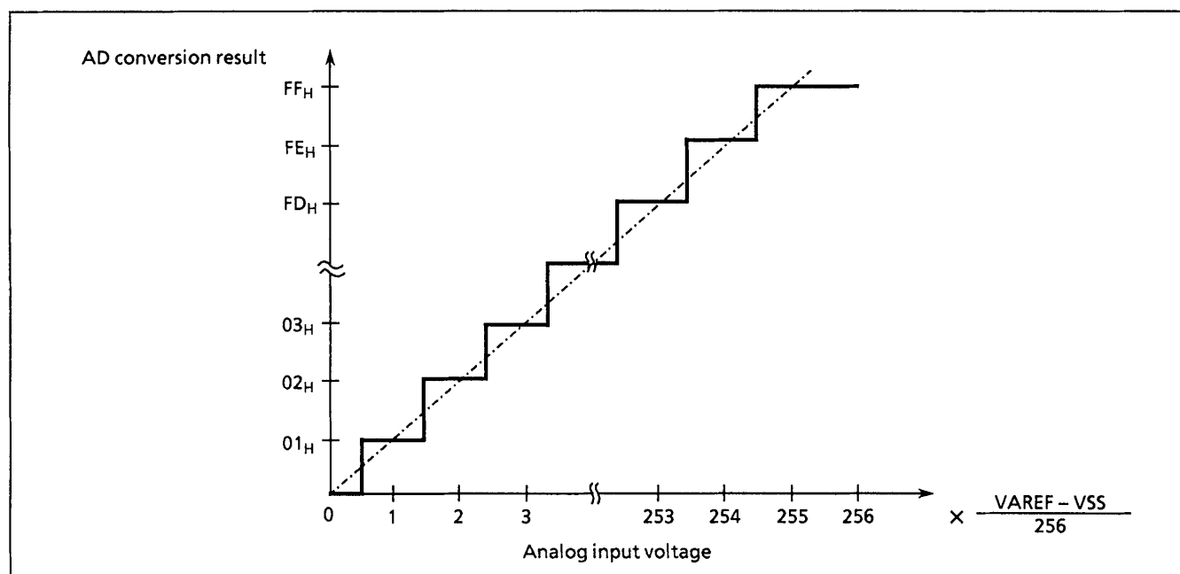
Figure 2-50. Analog Input Voltage and AD Conversion Result (typ.)
