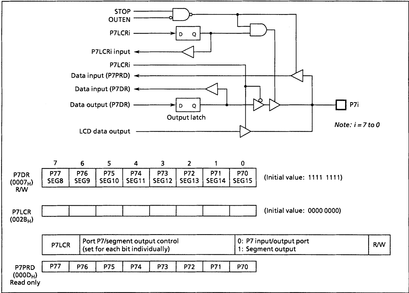
Figure 2-8. Port 7
