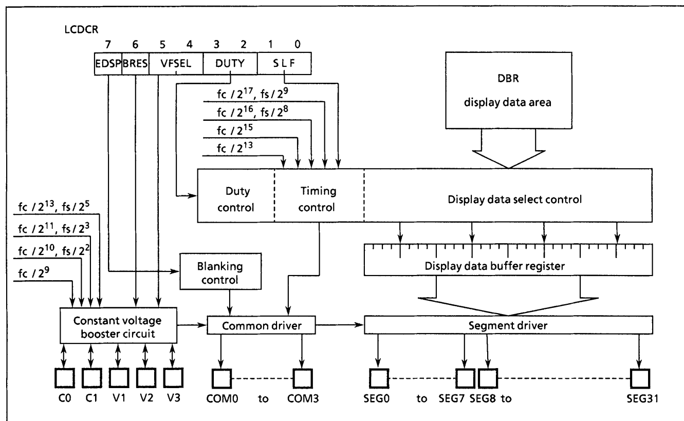
Figure 2-54. LCD Driver
