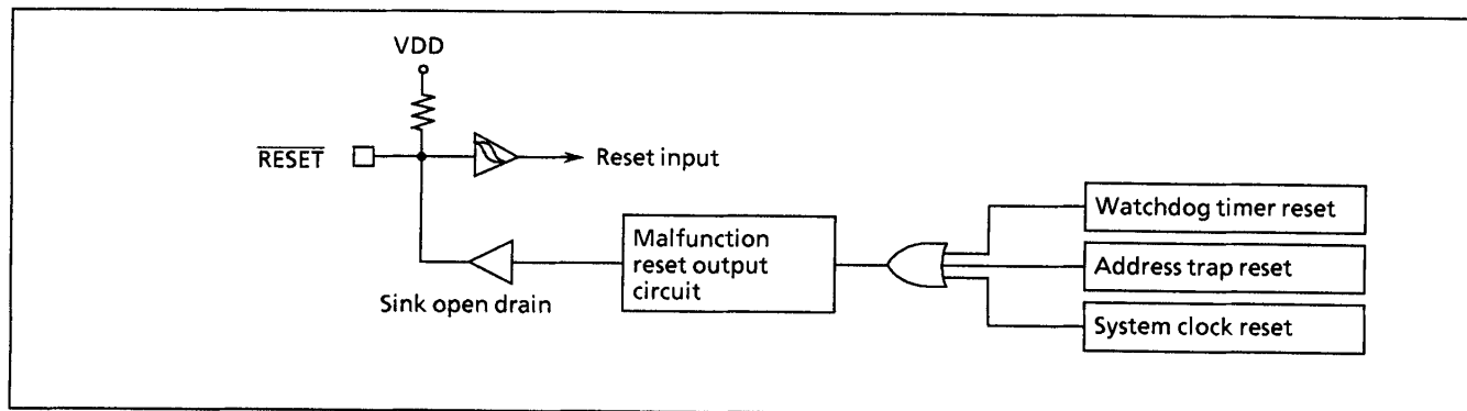
Figure 1-23. Reset Circuit
