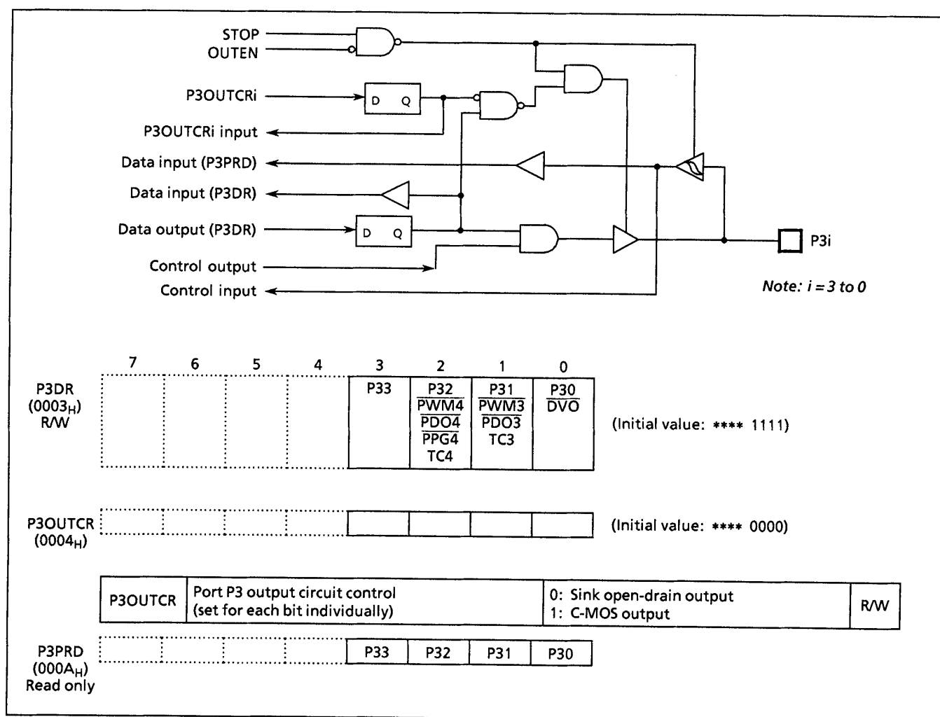
Figure 2-5. Port 3
