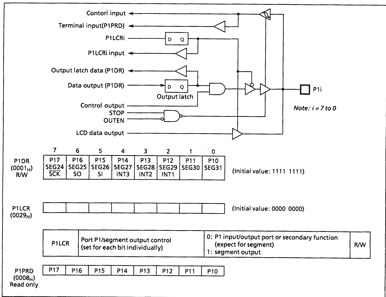
Figure 2-3. Port 1
