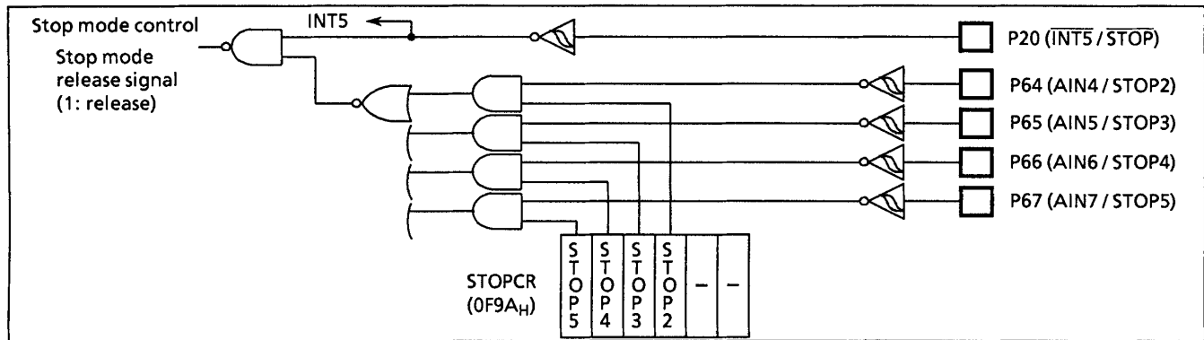
Figure 2-52. Stop Mode Control Circuit
