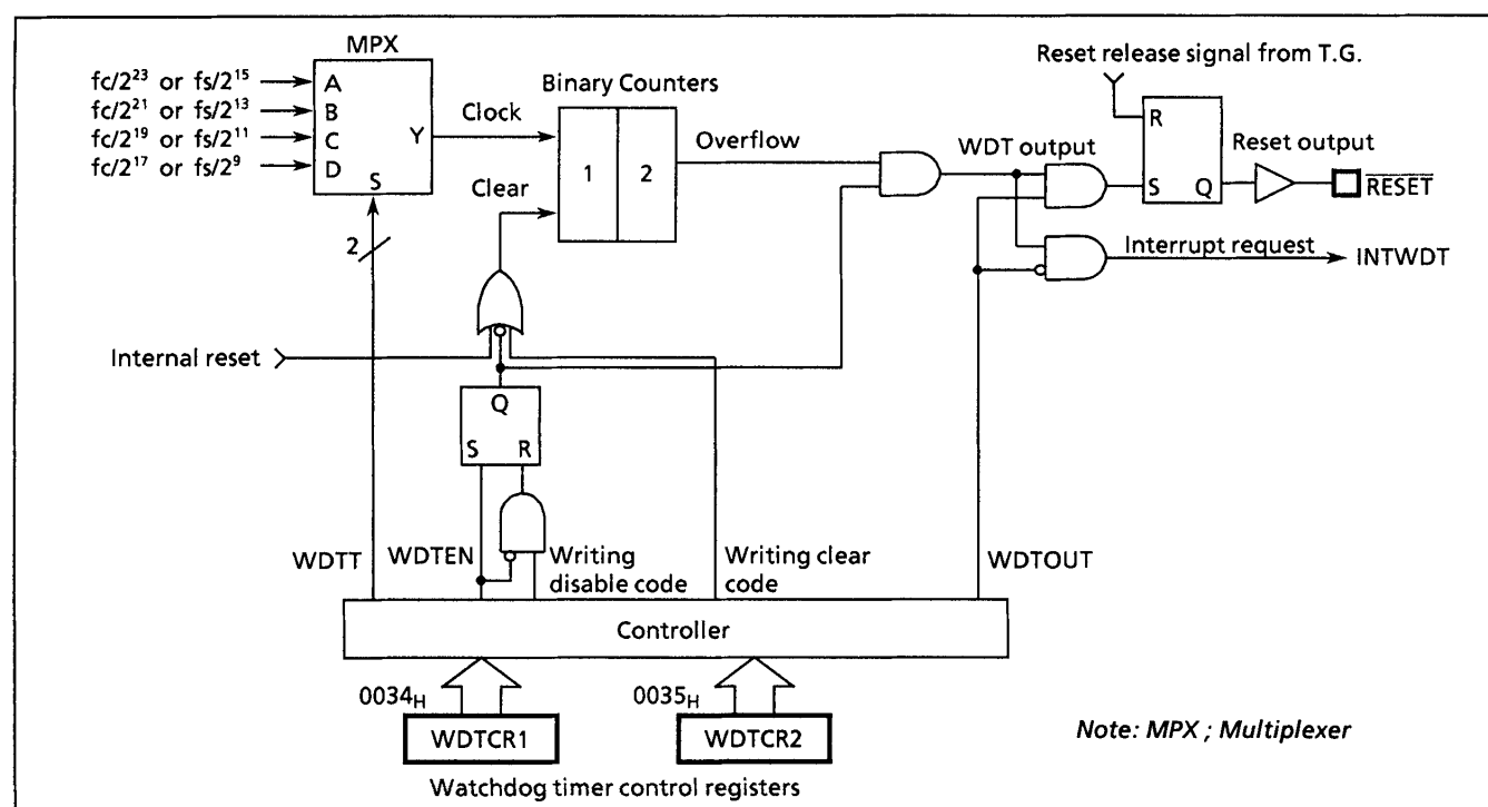
Figure 2-11. Watchdog Timer Configuration
