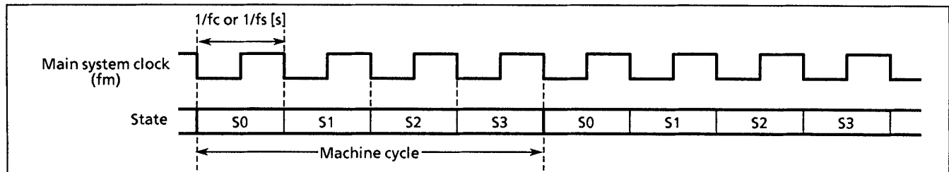
Figure 1-6. Machine Cycle
