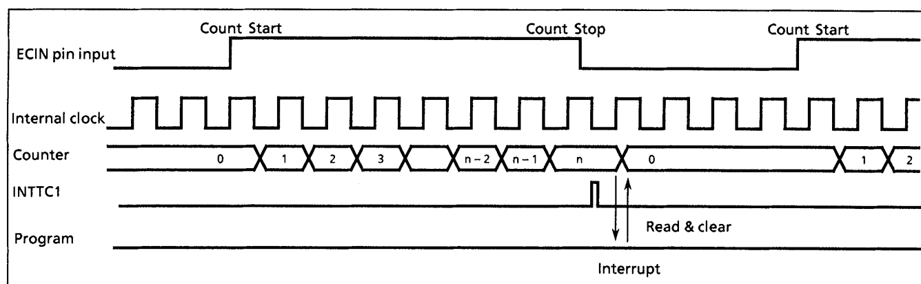
Figure 2-22. Pulse Width Measurement Mode Timing Chart
