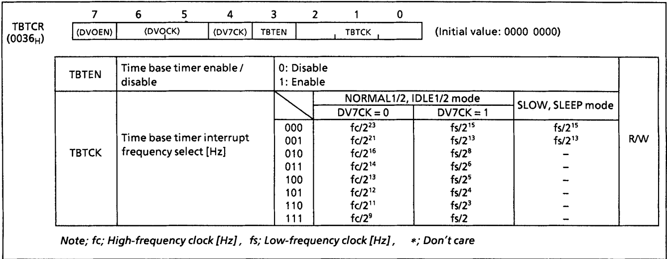
Figure 2-10. Time Base Timer Control Register
