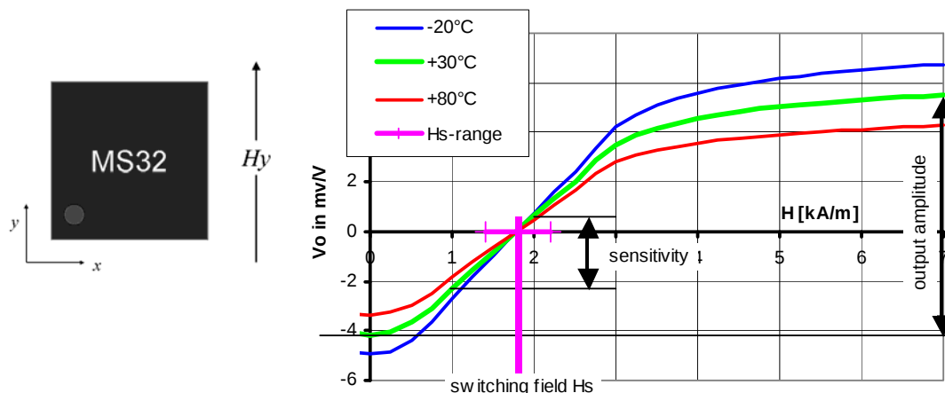
Figure 1: Characteristic curves for MS32 at different ambient temperatures (-20°C, +30°C, +80°C)
