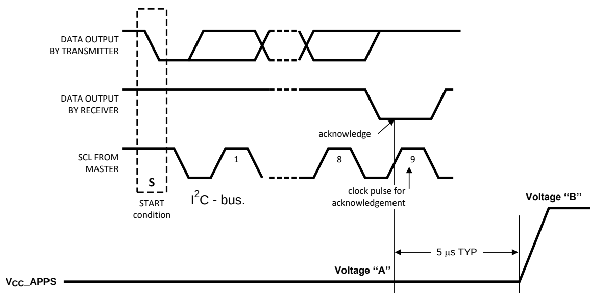
Figure 22. I²C DVM Timing For V CC_APPS (Buck1)
